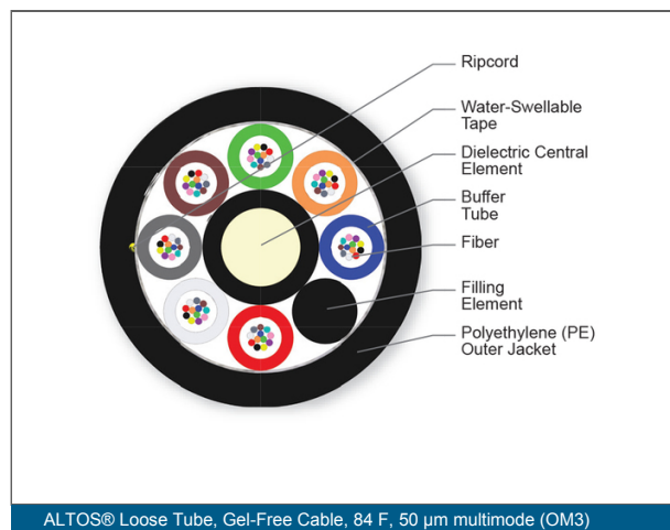
ALTOS® Loose Tube, Gel-Free Cable, 84 F, 50 µm multimode (OM3)
